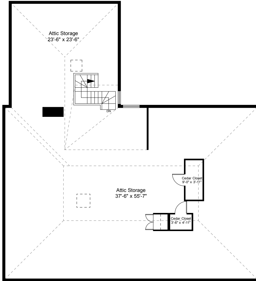
Attic Plan Ceiling Height = 9'-4"
